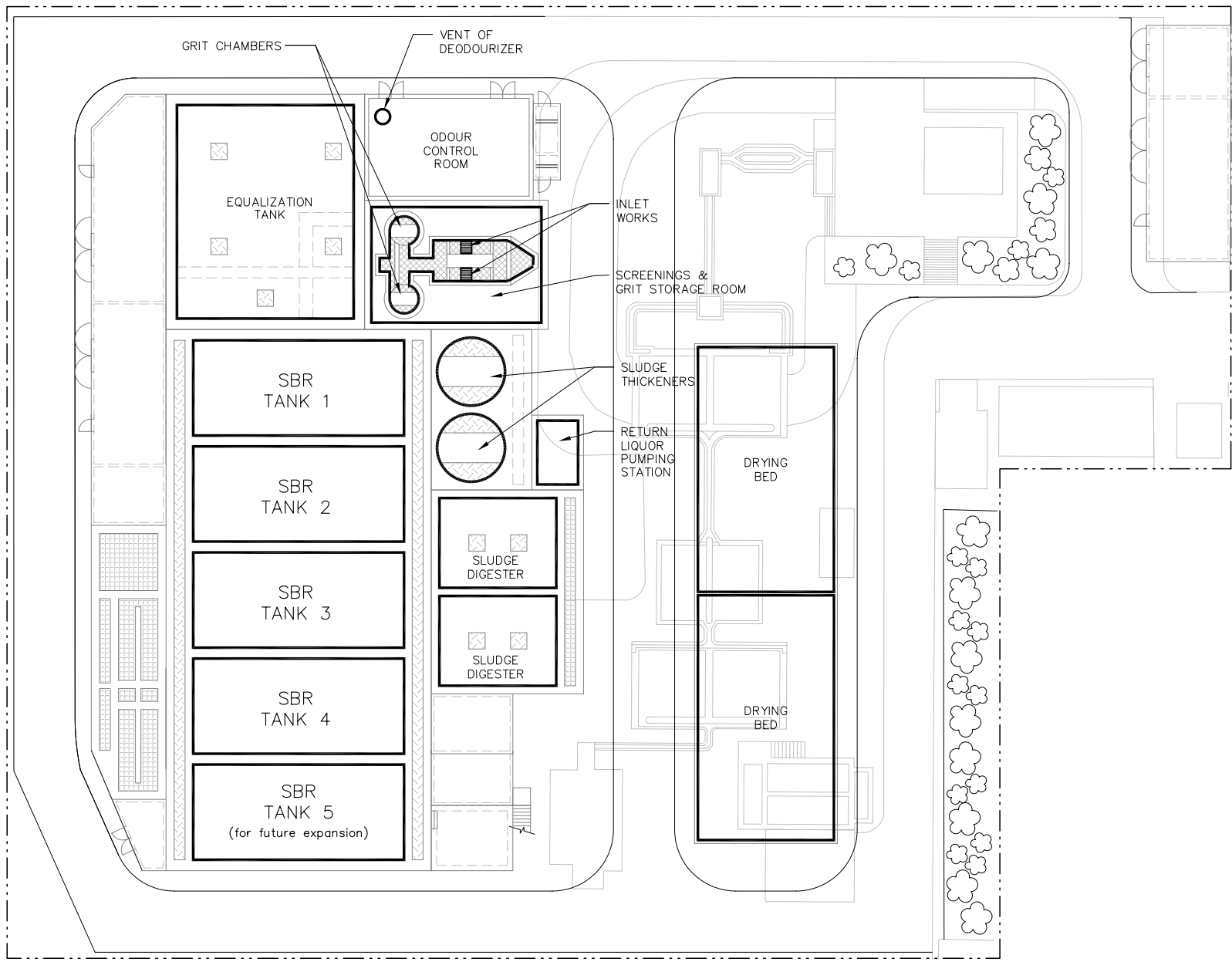
Figure 3-3 Location of Major Odour Emission Sources
